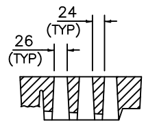
SECTION-DD.
