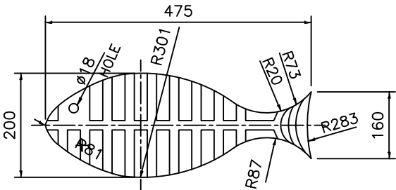
FISH DETAIL
