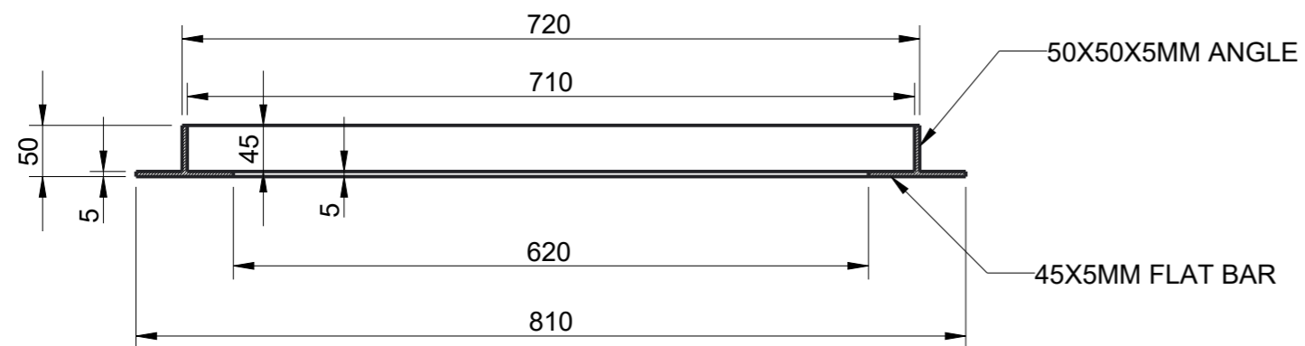
SECTION B-B
