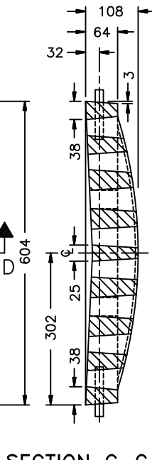
SECTION C-C
