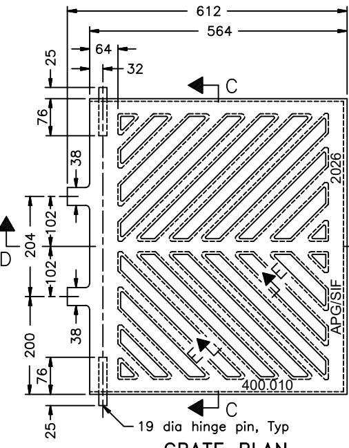
GRATE PLAN
