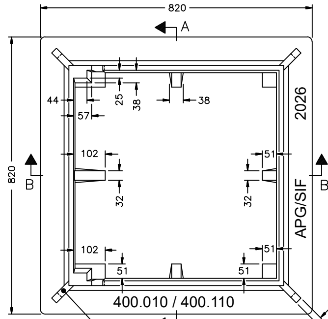
FRAME PLAN
