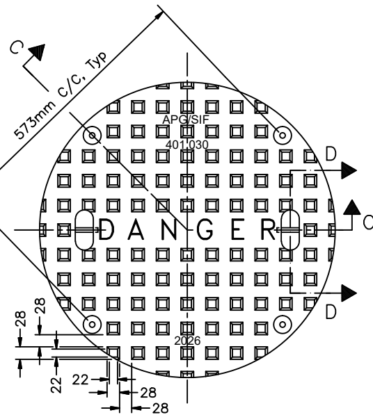
COVER PLAN
