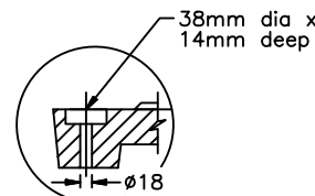
HOLE DETAIL
