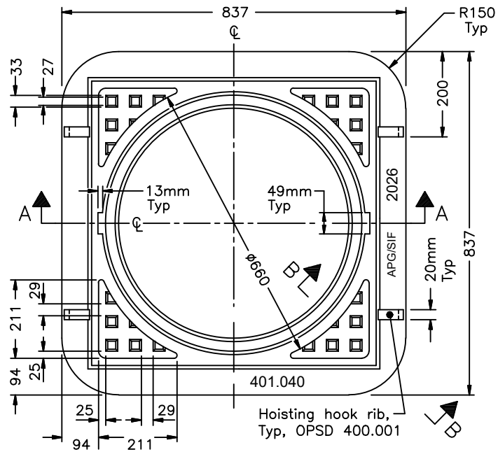
FRAME PLAN
