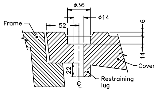
SECTION A-A FRAME WITH COVER SHOWN
