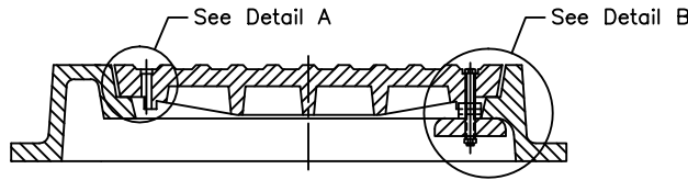
SECTION A-A FRAME WITH COVER SHOWN
