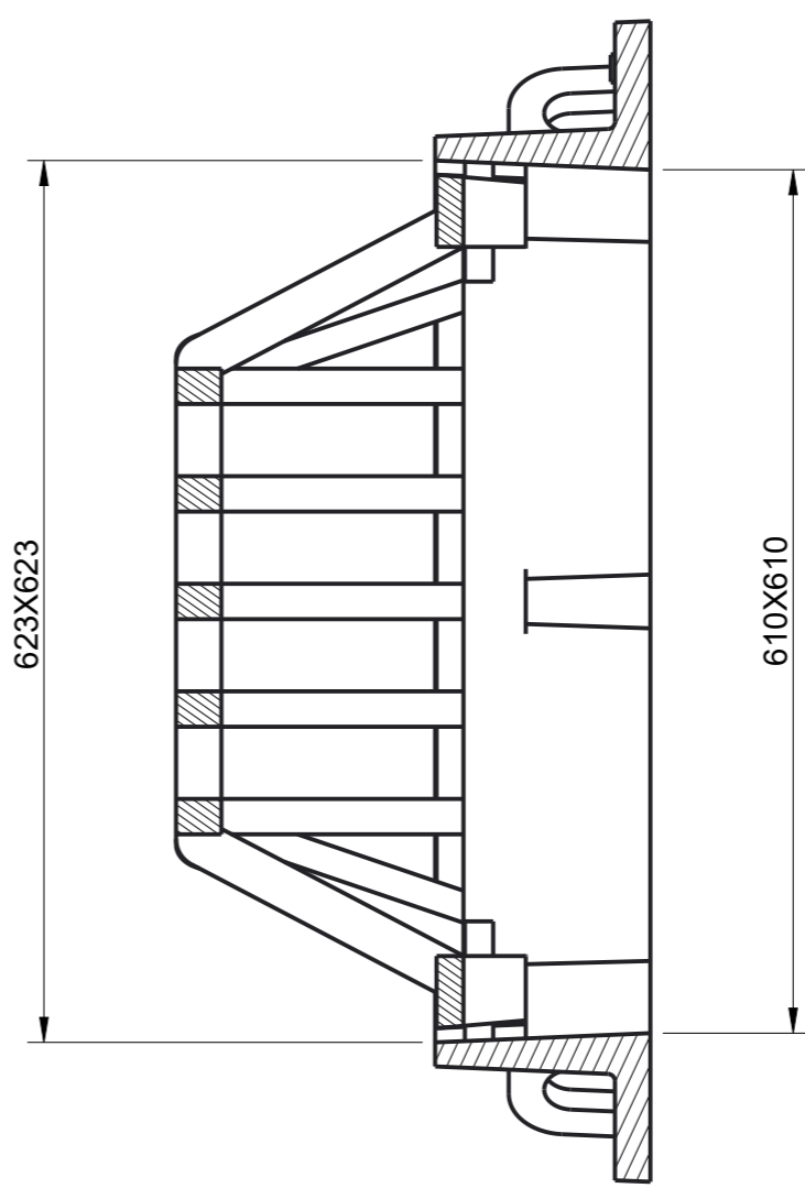
SECTION B-B
