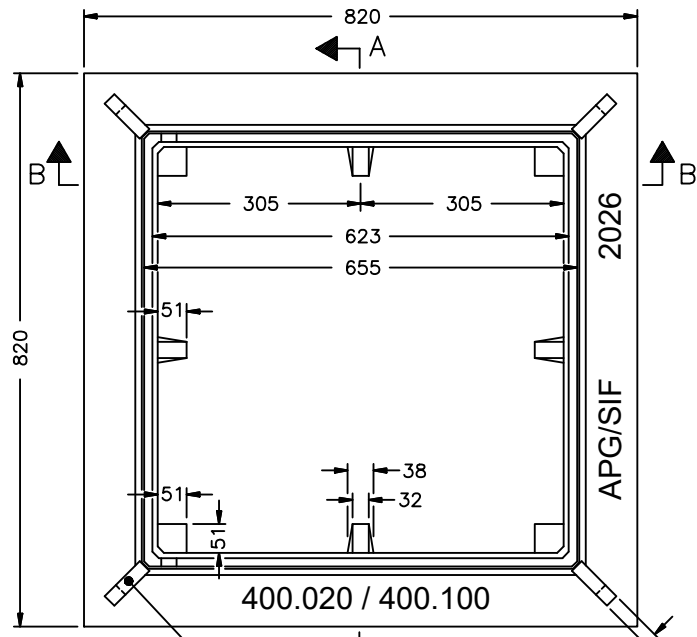
FRAME PLAN
