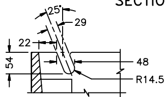
SLOT DETAIL
