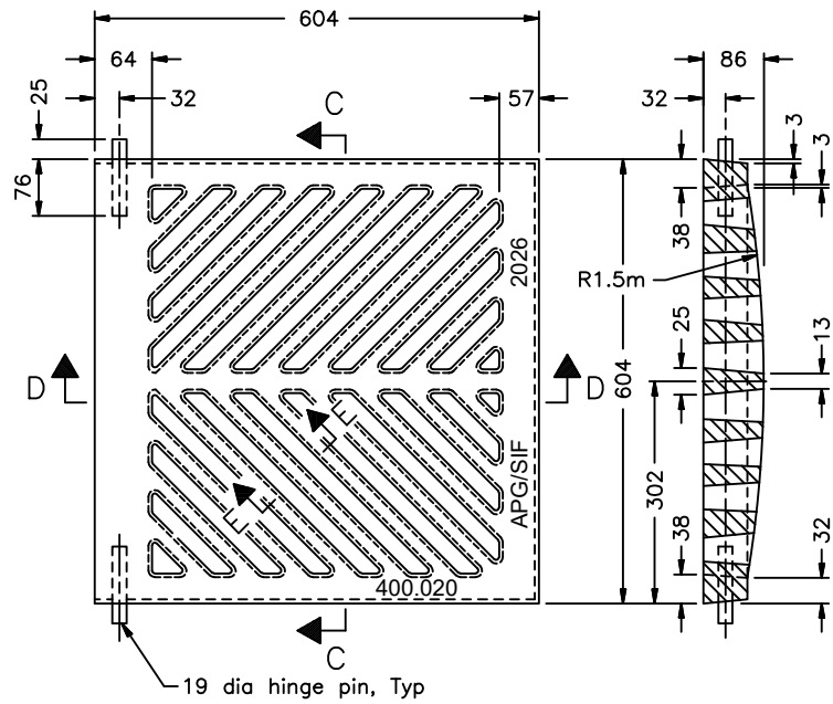
GRATE PLAN
