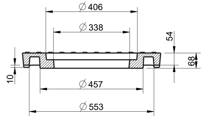
SECTION C-C OUTTER COVER
