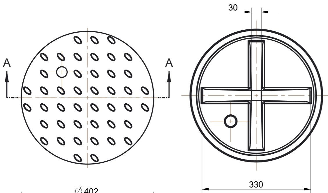
COVER BOTTOM VIEW
