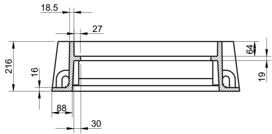
SECTION B-B FRAME VIEW
