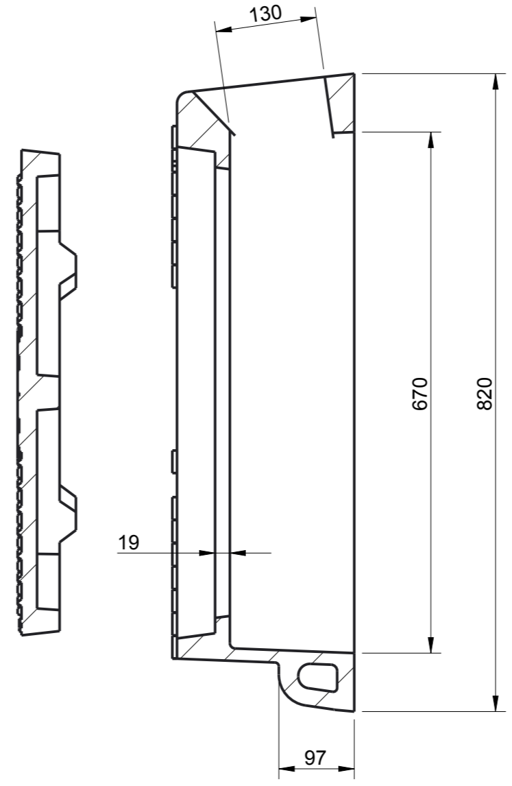
SECTION B-B
