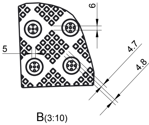
Dome Design Detail
