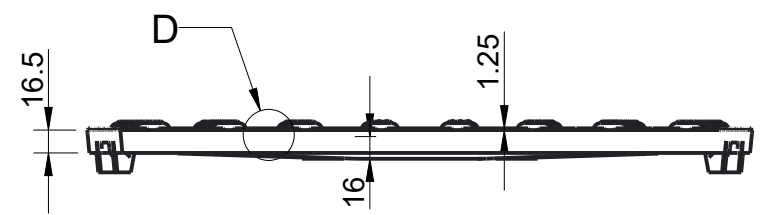
SECTION F-F
