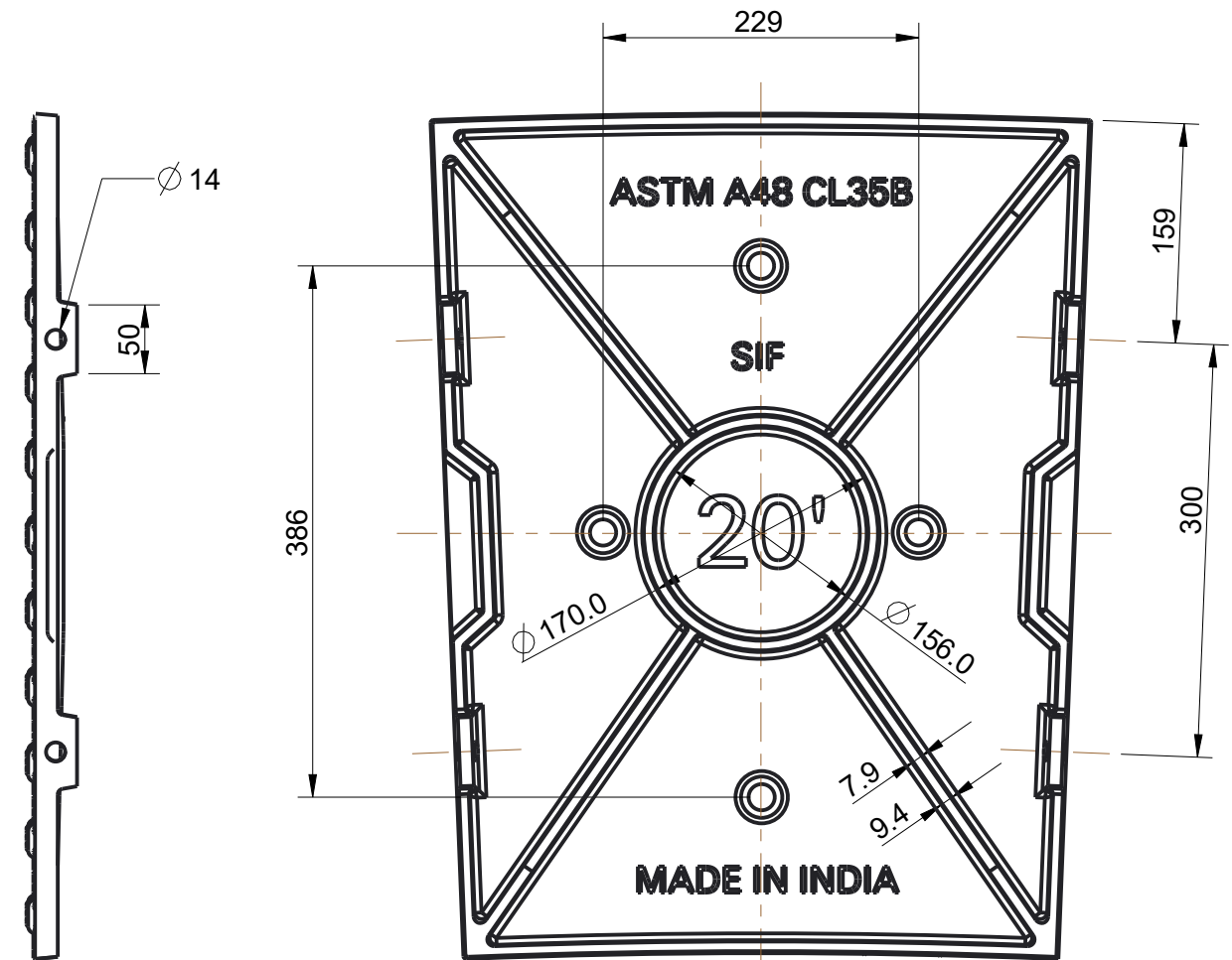
BOTTOM VIEW
