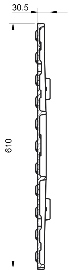
SECTION B-B
