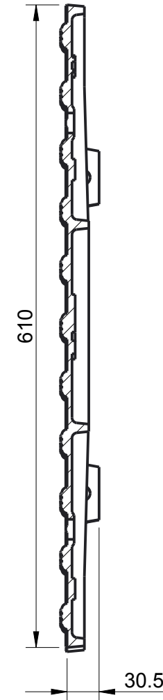
SECTION B-B
