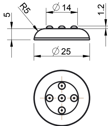
Dome Design Detail
