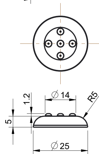
DOME DETAILS
