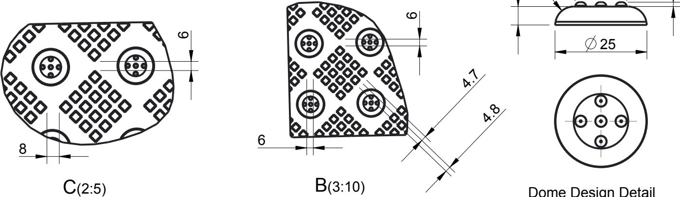
Dome Design Detail
